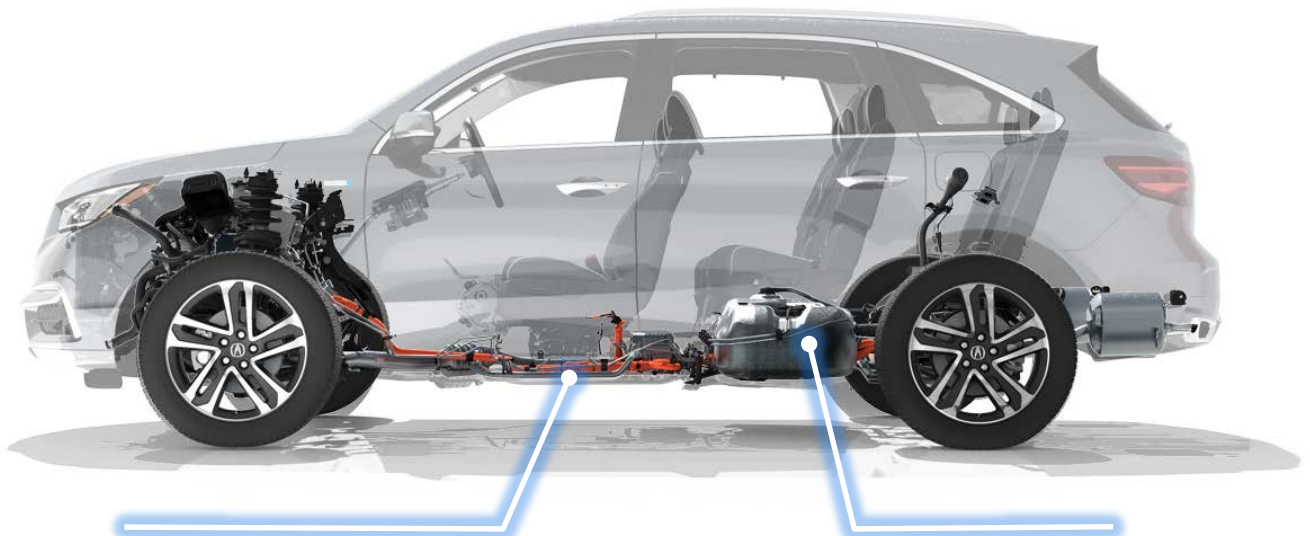
High-Voltage Cables
